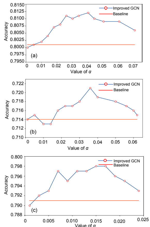
Fig. 3 Node classification prediction accuracy on the Cora (a), Citeseer (b), and Pubmed (c) datasets with changing \alpha
